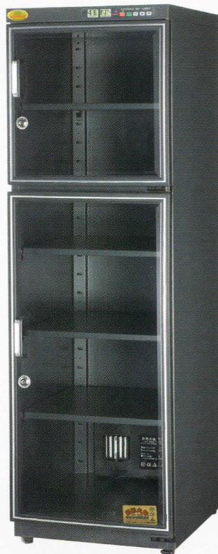
DRY-205 EX: W400 × D530 × H1292mm IN: W398 × D475 × H1210mm CAPACITY: 228L SHELF: 5PCS WEIGHT: 30KGS MAX/AVG 30W/12W
